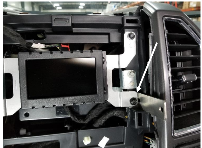
Loosen (2) OEM fasteners on the right of the display and attach side mounting bracket.
