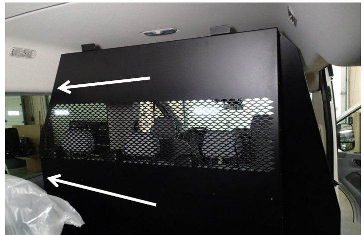
Attach driver side upper and lower side filler panels using five (5) 1/4 x 3/4" carriage bolts and serrated nuts. Filler panels angle toward front of vehicle
