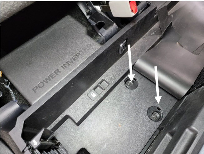
Remove cover plates to expose fasteners.
