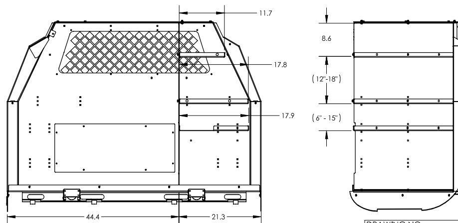
(DRIVER SIDE-SHOWN) ILLUSTRATION # 4 ASSEMBLED FRONT BULKHEAD AND DRAWER IS NOT SHOWN FOR CLARITY
