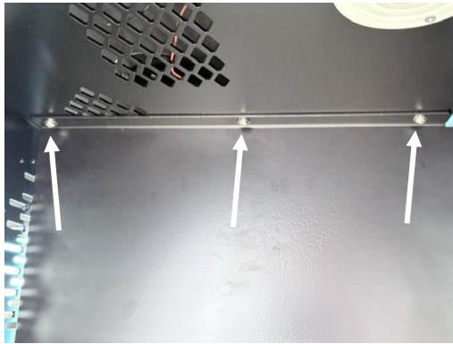
Loosely attach divider (56727/56728) to ceiling using three (3) 1/4" x 3/4" Phillips pan head machine
