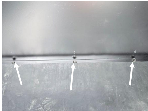
Once everything is tight, secure bottom of divider of K9 floor using three (3) 1/4" x 3/4" self-threading screws.
