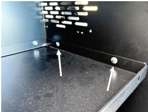
Loosely attach top shelf to rear bulkhead using two (2) 1/4" x 1/2" carriage bolts and serrated nuts.
