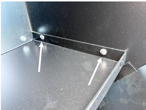
Loosely attach bottom shelf to rear bulkhead two (2) 1/4" x 1/2" carriage bolts and serrated nuts.
