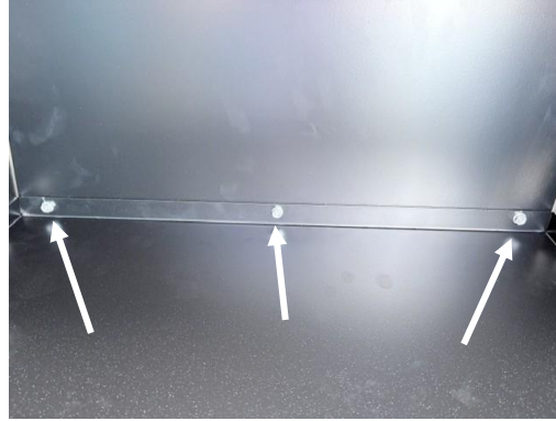
Loosely attach bottom shelf (56731/56732) to divider using three (3) 1/4" x 1/2" carriage bolts (inserted from
