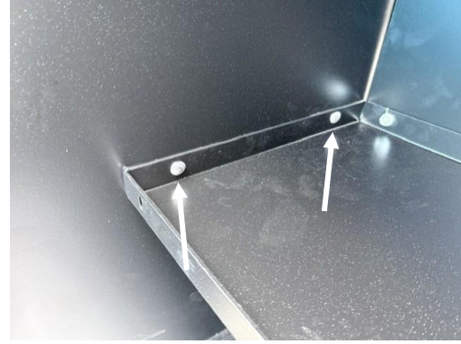
Loosely attach bottom shelf to front bulkhead using three (3) 1/4" x 1/2" carriage bolts and serrated nuts.
