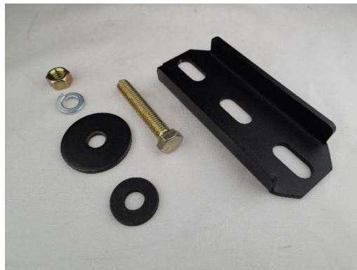
KKM007376 Backing plate and other bulkhead to floor mount hardware shown.
