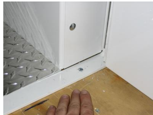
Repeat for other side and the front bulkhead to keep the assembly square.
