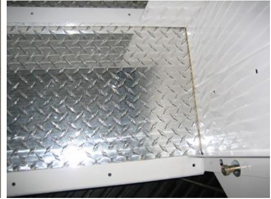
Screw down third compartment door frame with #10 x1-1/4" Phillips screws and install cover over third compartment bench.
