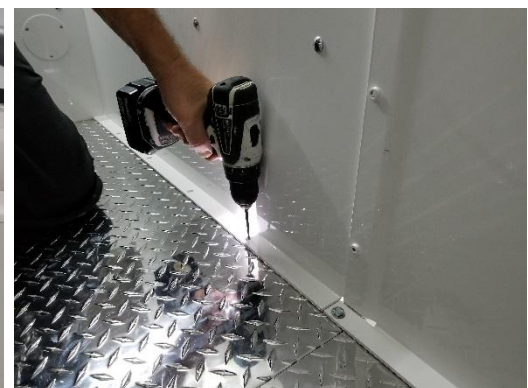
Center and straighten the divider and drill 3/16" holes through diamond plate only . Do not drill through OEM van floor.
